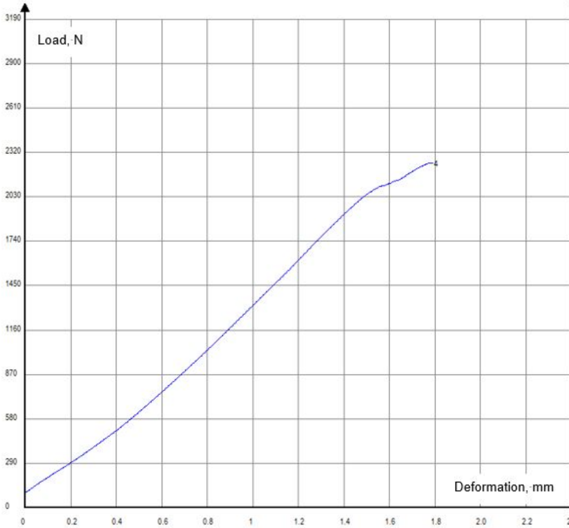
Test Curve – Specimen No. 4
