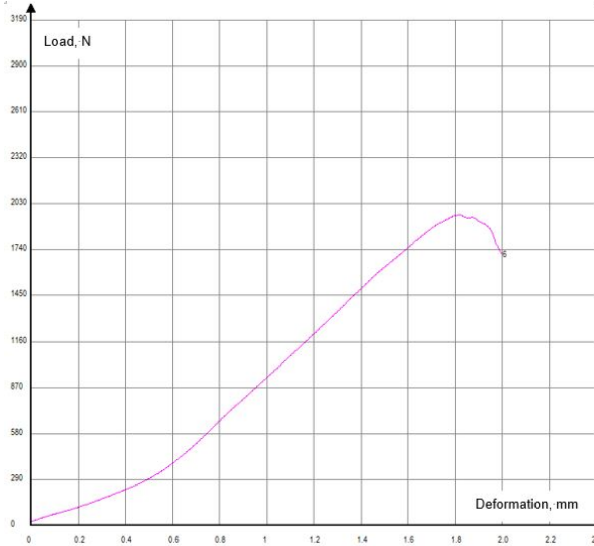
Curve – Specimen No. 6
