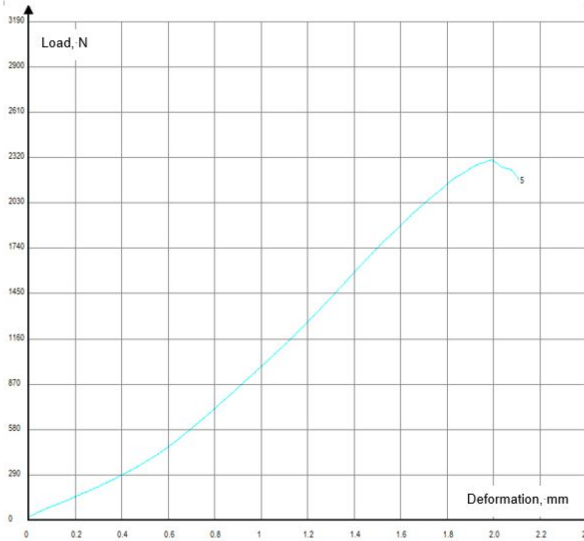
Test Curve – Specimen No. 5
