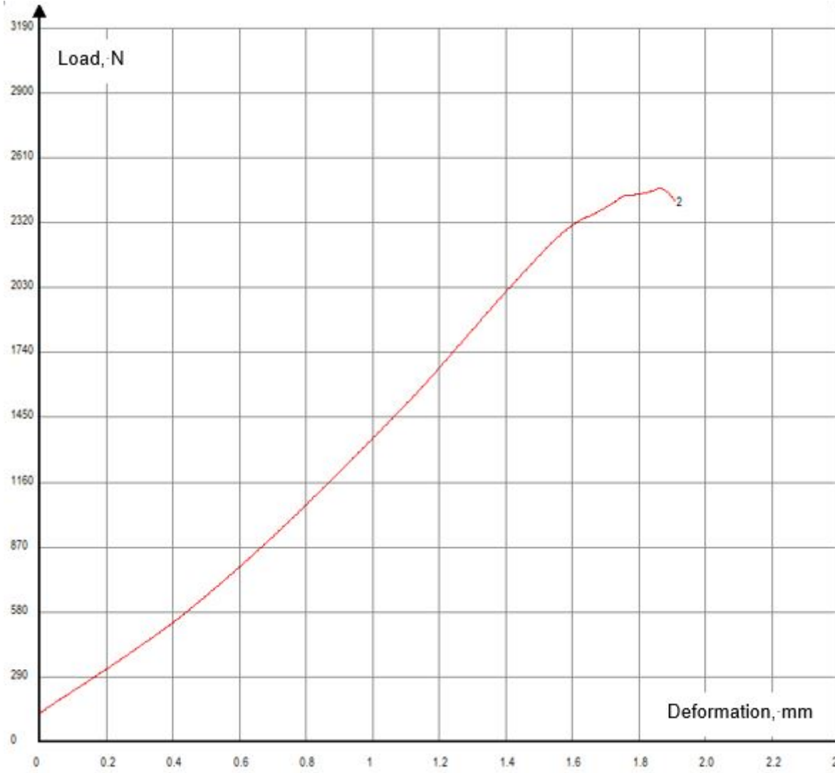
Test Curve – Specimen No. 2
