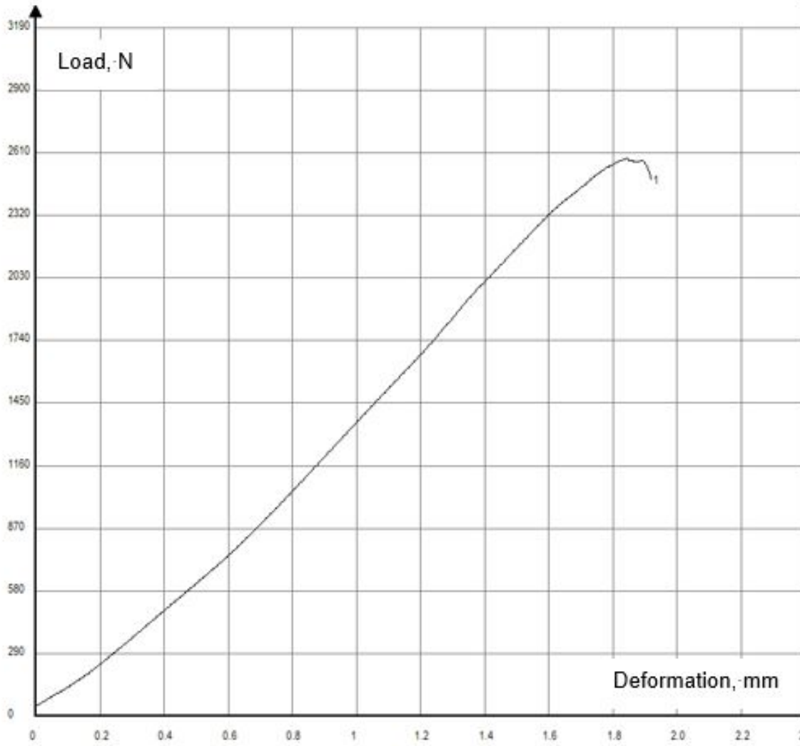
Test Curve – Specimen No. 1
